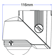
Eave mount
