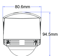
Wall mount
